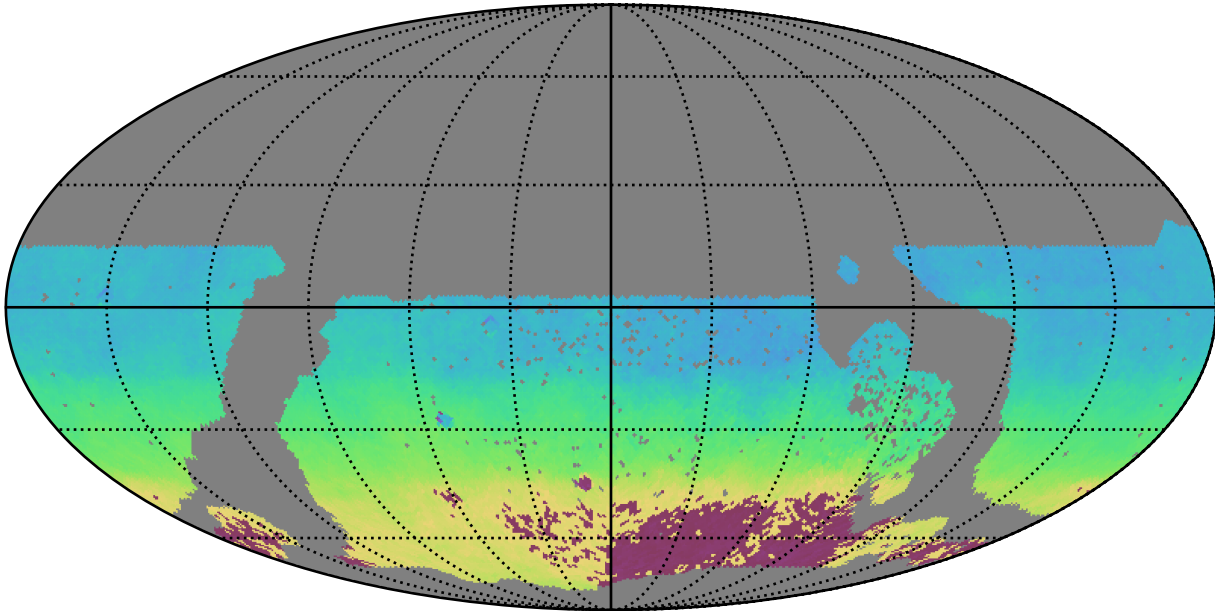
early_ss_template_fpextra2.0_v3.4_10yrs WFD y band: AngleMean rotSkyPos
