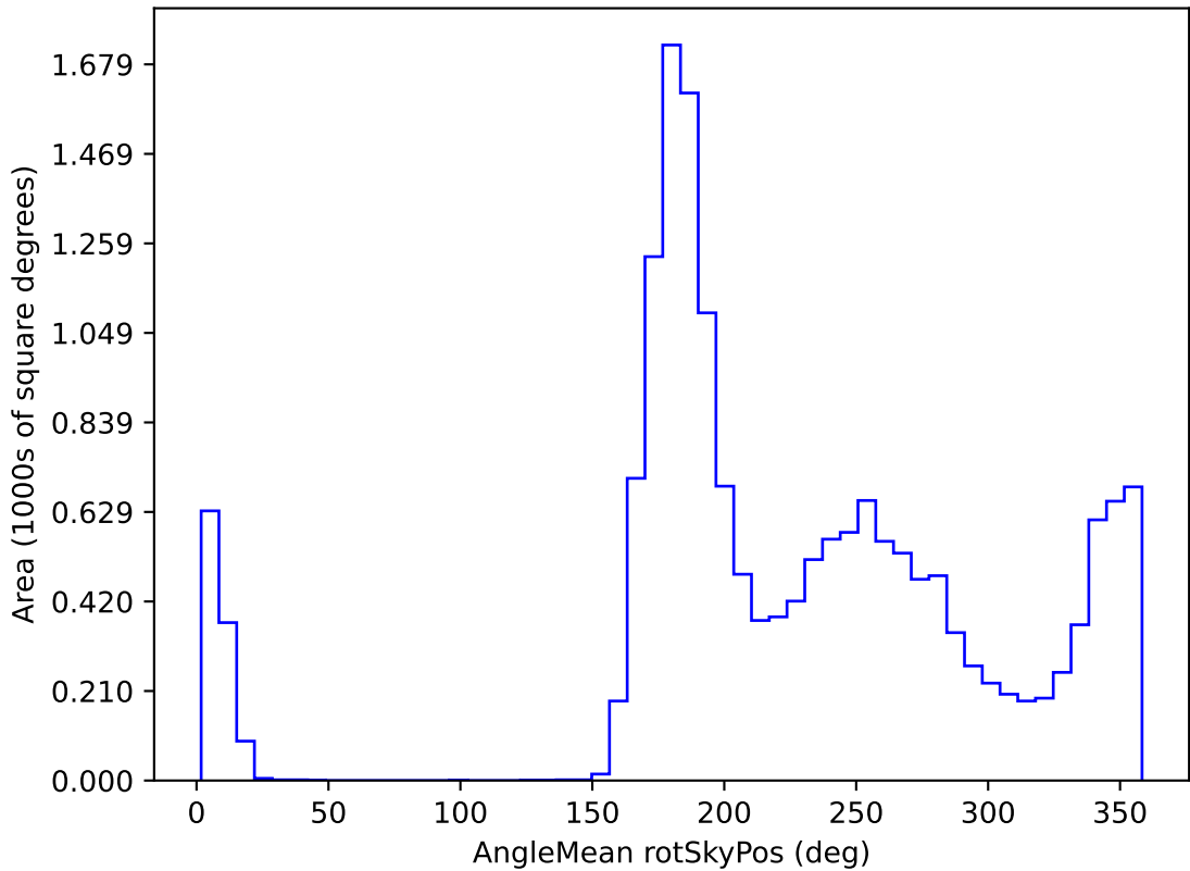
early_ss_template_fpextra2.0_v3.4_10yrs WFD y band: AngleMean rotSkyPos
