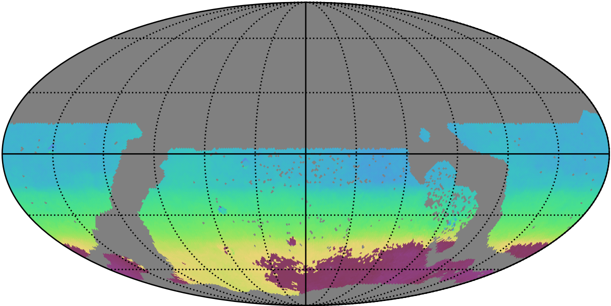
early_ss_template_fpextra2.0_v3.4_10yrs WFD all bands: AngleMean rotSkyPos
