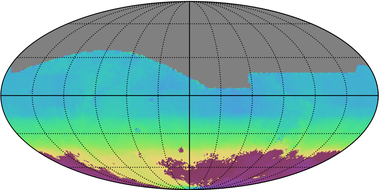
early_ss_template_fpextra2.0_v3.4_10yrs All sky all bands: AngleMean rotSkyPos
