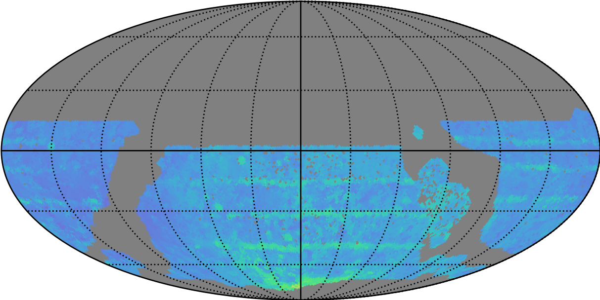
early_ss_template_fpextra2.0_v3.4_10yrs WFD z band: 80thPercentile Season Length
