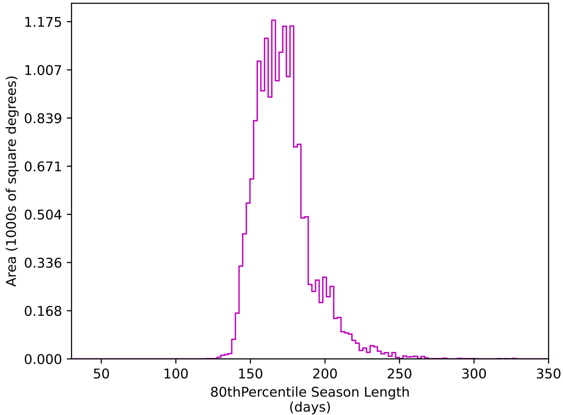
early_ss_template_fpextra2.0_v3.4_10yrs WFD z band: 80thPercentile Season Length
