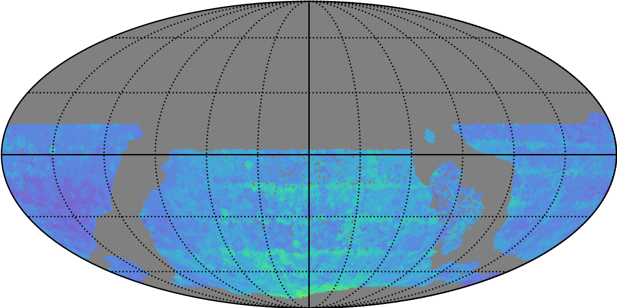
early_ss_template_fpextra2.0_v3.4_10yrs WFD y band: 80thPercentile Season Length
