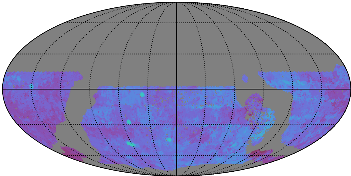
early_ss_template_fpextra2.0_v3.4_10yrs WFD u band: 80thPercentile Season Length
