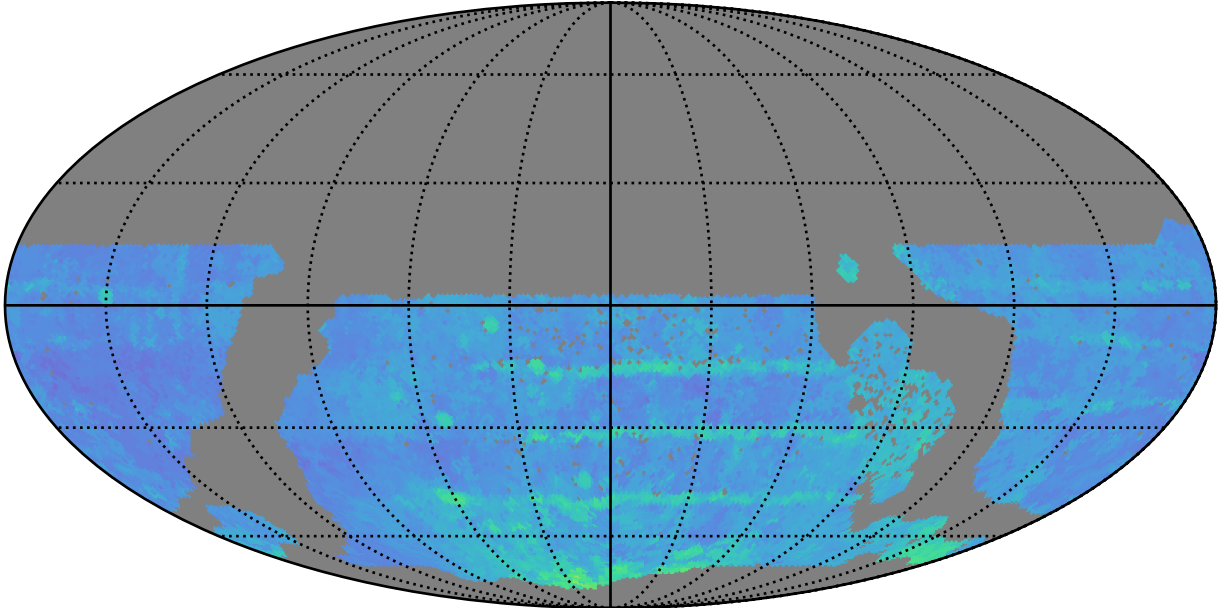
early_ss_template_fpextra2.0_v3.4_10yrs WFD r band: 80thPercentile Season Length
