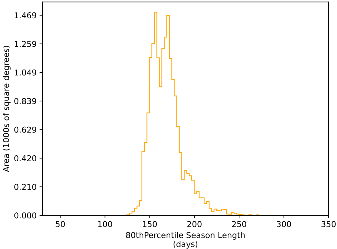
early_ss_template_fpextra2.0_v3.4_10yrs WFD r band: 80thPercentile Season Length
