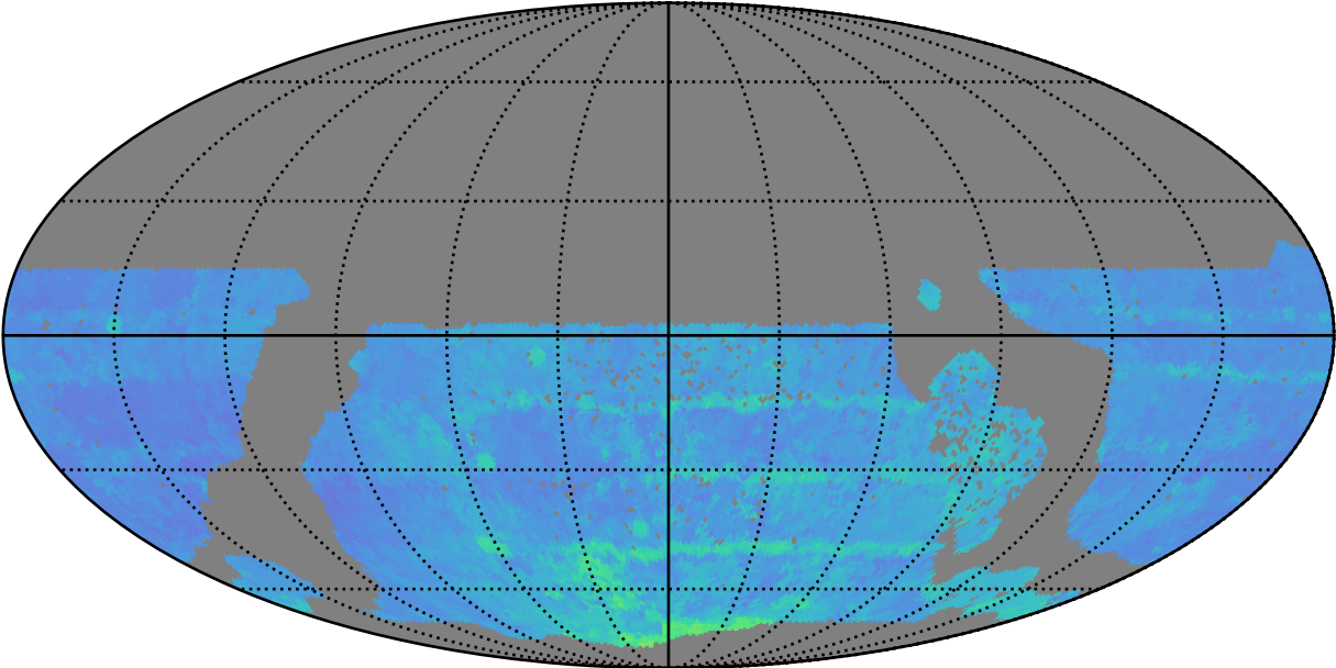
early_ss_template_fpextra2.0_v3.4_10yrs WFD i band: 80thPercentile Season Length
