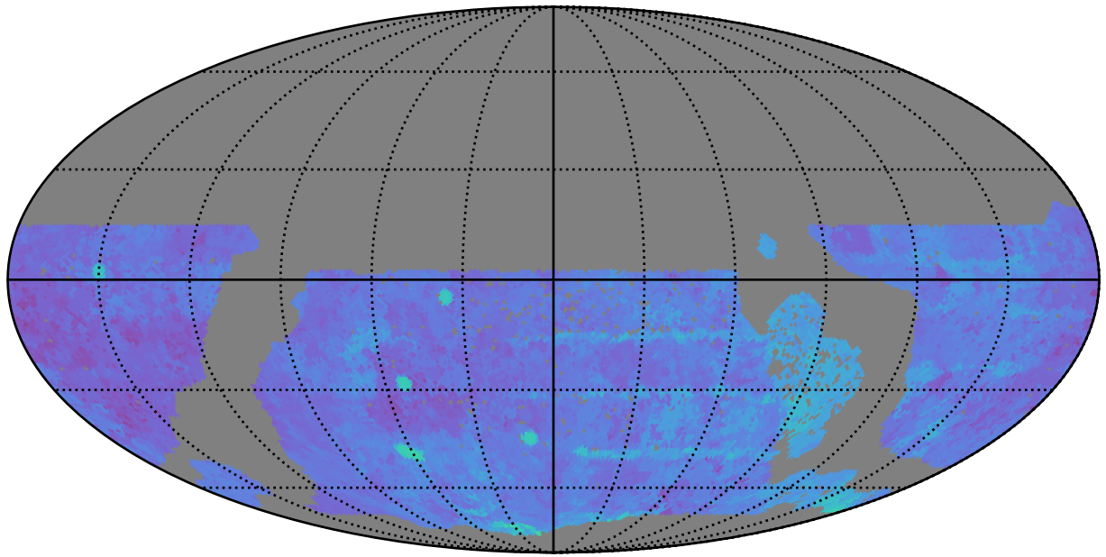
early_ss_template_fpextra2.0_v3.4_10yrs WFD g band: 80thPercentile Season Length
