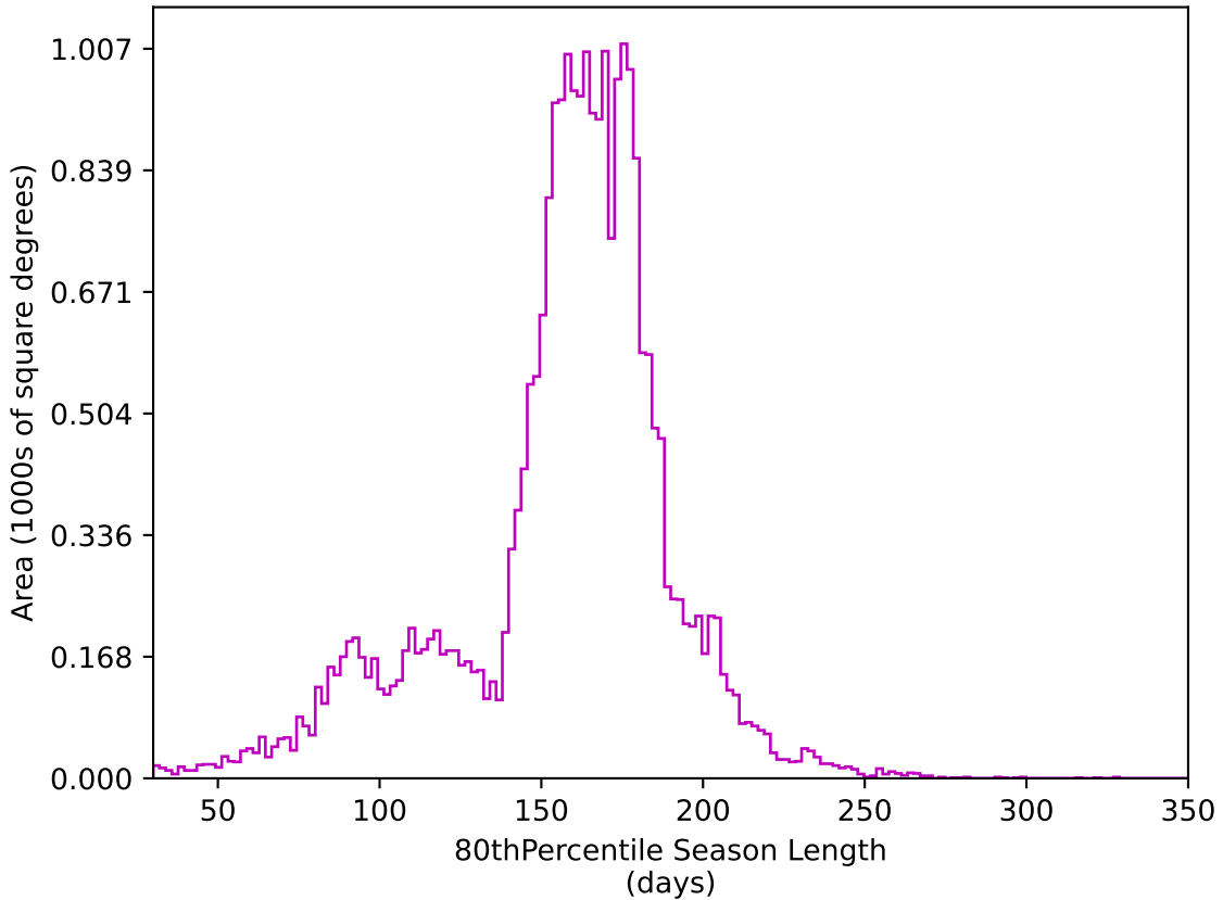
early_ss_template_fpextra2.0_v3.4_10yrs All sky z band: 80thPercentile Season Length
