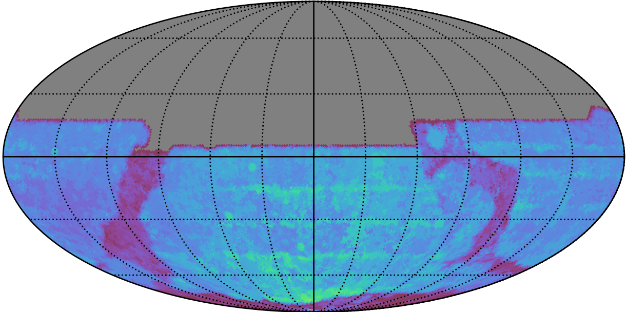
early_ss_template_fpextra2.0_v3.4_10yrs All sky y band: 80thPercentile Season Length
