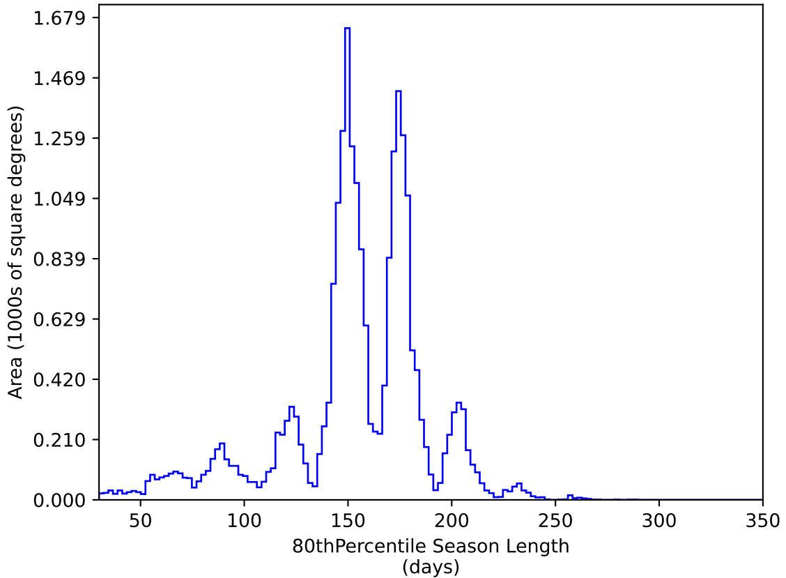
early_ss_template_fpextra2.0_v3.4_10yrs All sky y band: 80thPercentile Season Length
