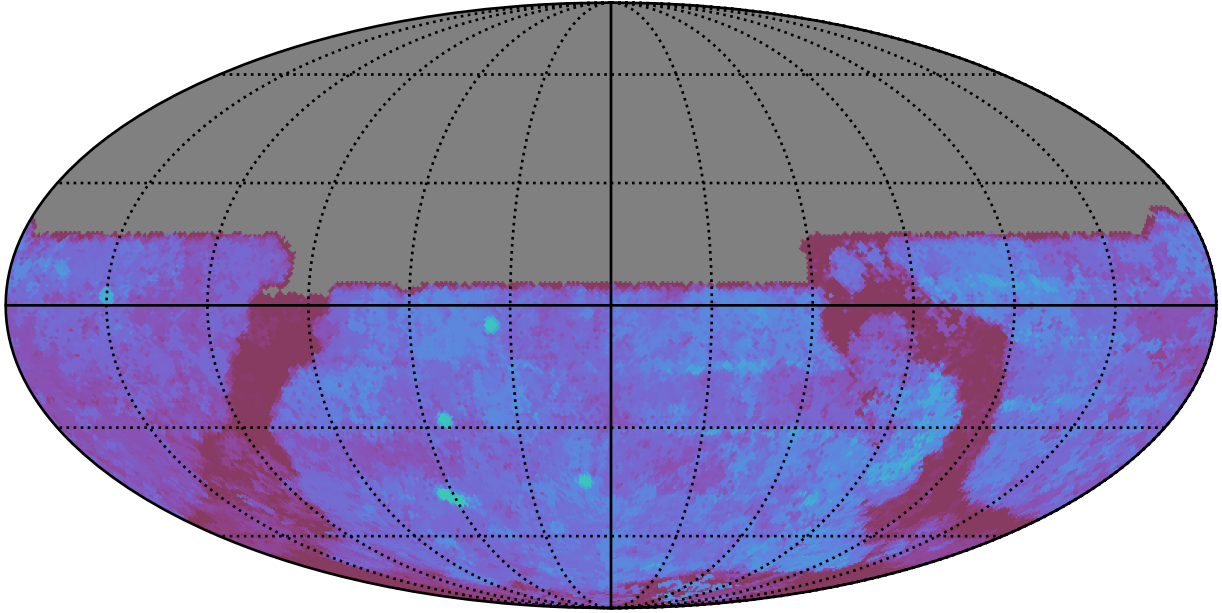
early_ss_template_fpextra2.0_v3.4_10yrs All sky u band: 80thPercentile Season Length
