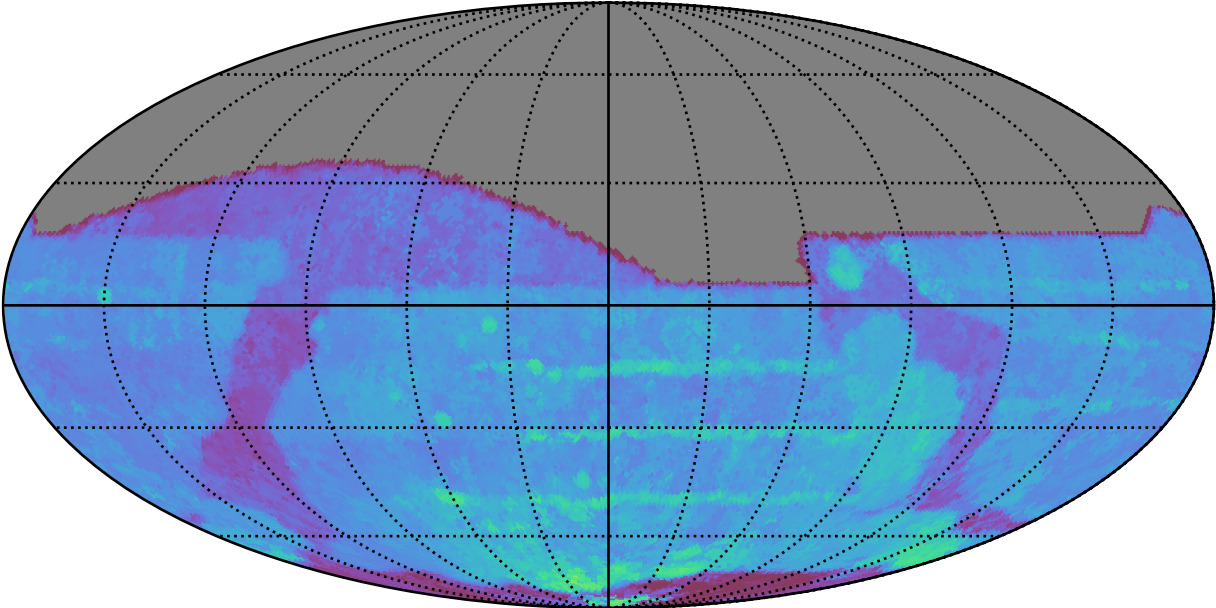
early_ss_template_fpextra2.0_v3.4_10yrs All sky r band: 80thPercentile Season Length
