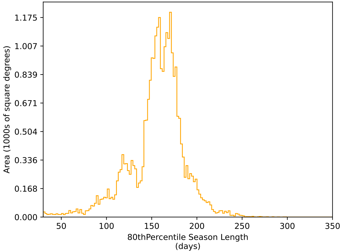
early_ss_template_fpextra2.0_v3.4_10yrs All sky r band: 80thPercentile Season Length
