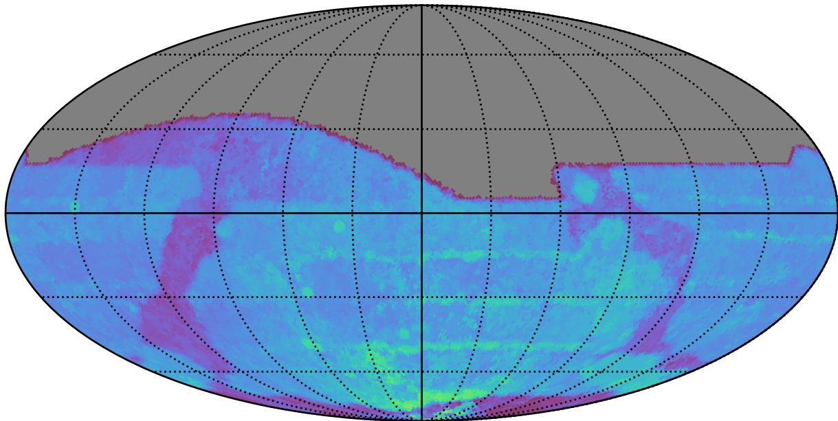
early_ss_template_fpextra2.0_v3.4_10yrs All sky i band: 80thPercentile Season Length
