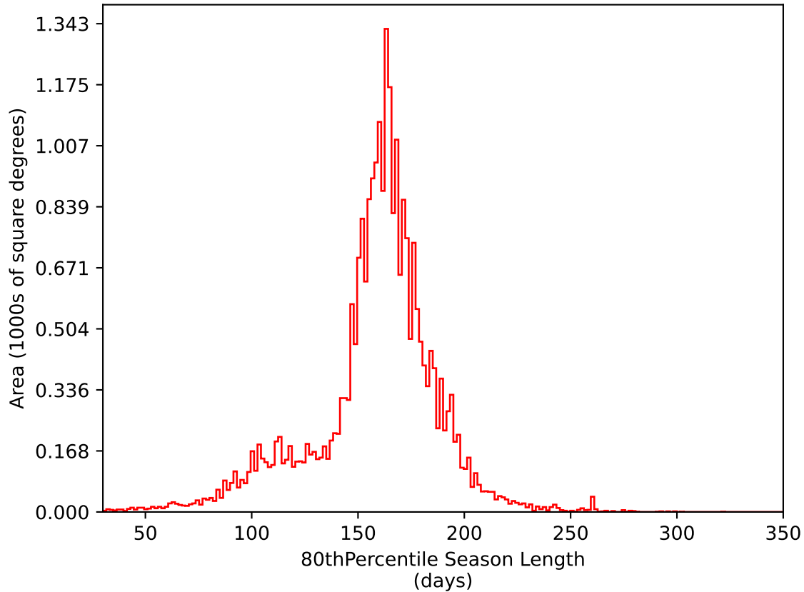
early_ss_template_fpextra2.0_v3.4_10yrs All sky i band: 80thPercentile Season Length
