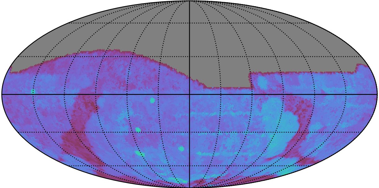
early_ss_template_fpextra2.0_v3.4_10yrs All sky g band: 80thPercentile Season Length
