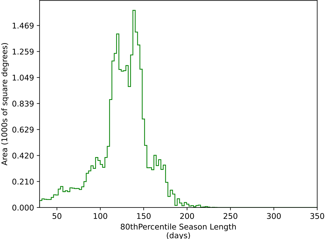
early_ss_template_fpextra2.0_v3.4_10yrs All sky g band: 80thPercentile Season Length
