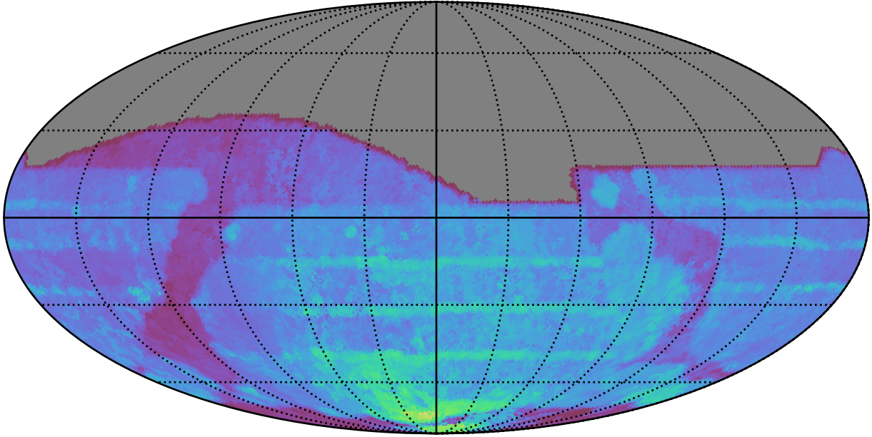
early_ss_template_fpextra2.0_v3.4_10yrs All sky all bands: 80thPercentile Season Length
