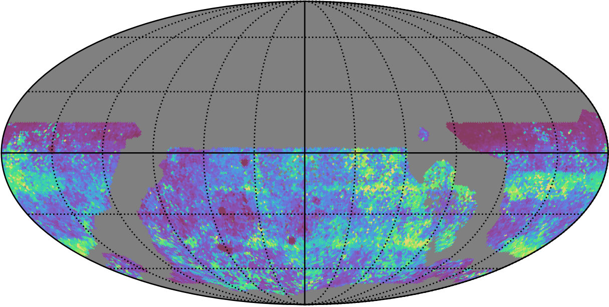
early_ss_template_fpextra2.0_v3.4_10yrs WFD zy bands: 75th Percentile Intranight Timespan
