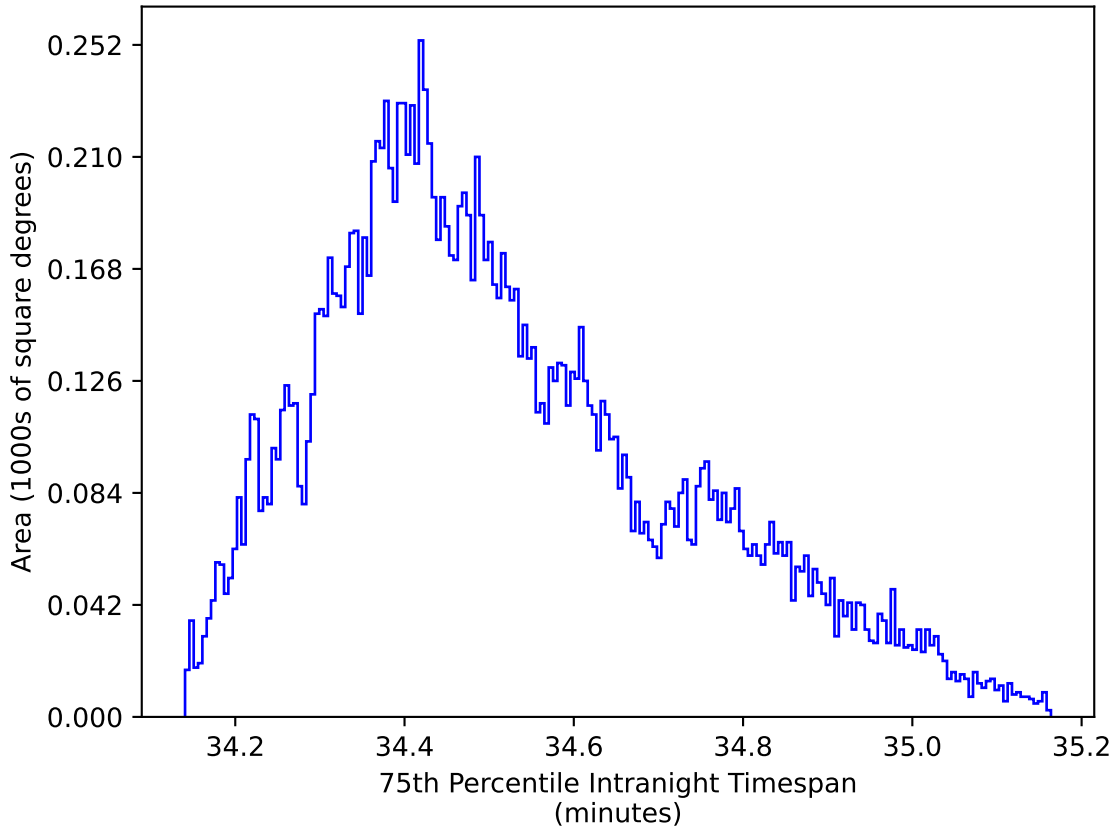
early_ss_template_fpextra2.0_v3.4_10yrs WFD zy bands: 75th Percentile Intranight Timespan
