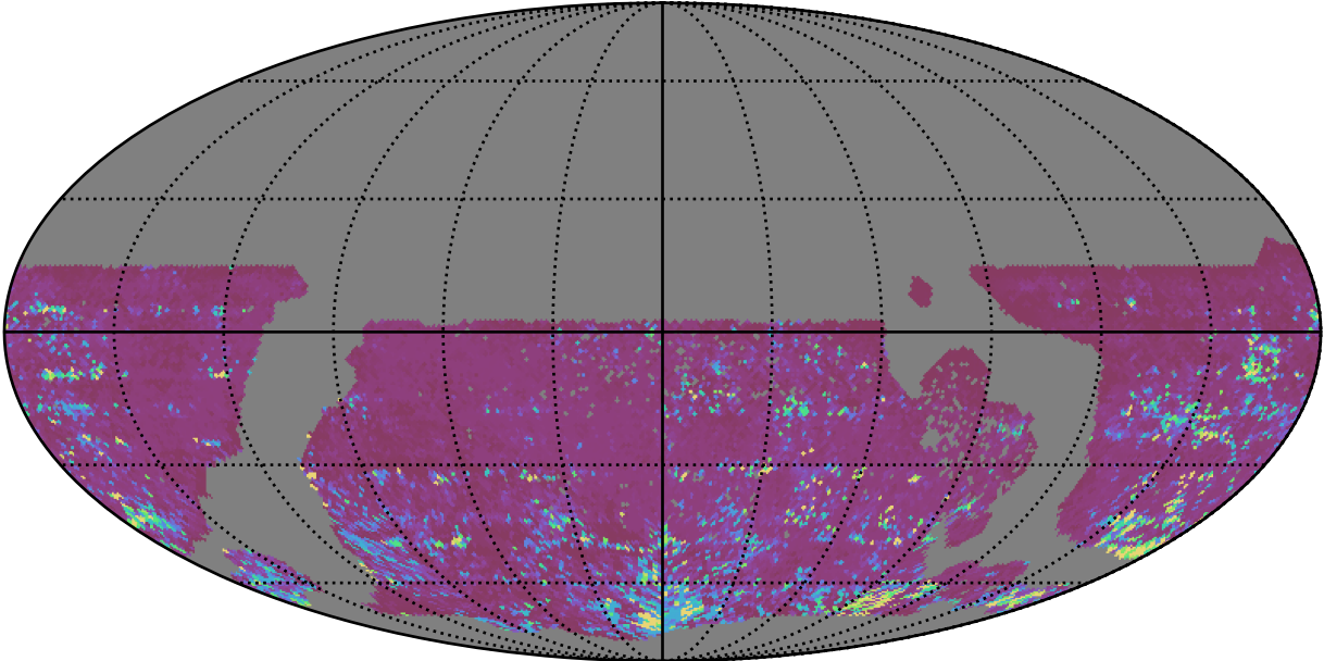
early_ss_template_fpextra2.0_v3.4_10yrs WFD z band: 75th Percentile Intranight Timespan
