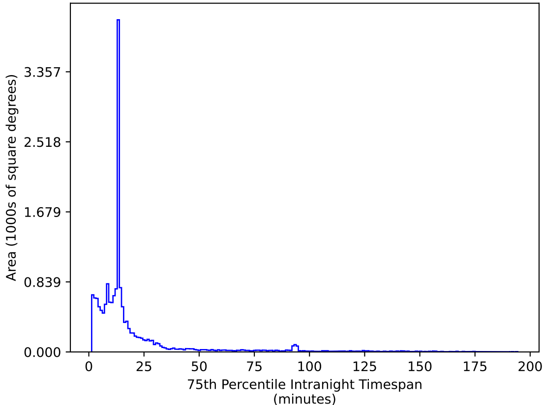
early_ss_template_fpextra2.0_v3.4_10yrs WFD z band: 75th Percentile Intranight Timespan
