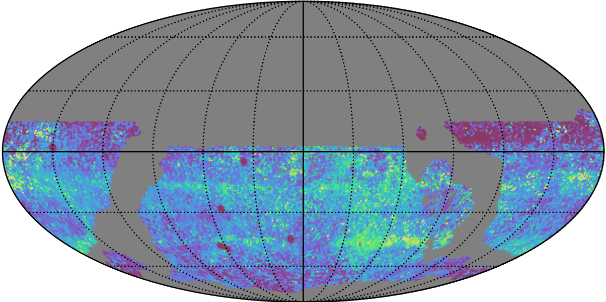
early_ss_template_fpextra2.0_v3.4_10yrs WFD y band: 75th Percentile Intranight Timespan
