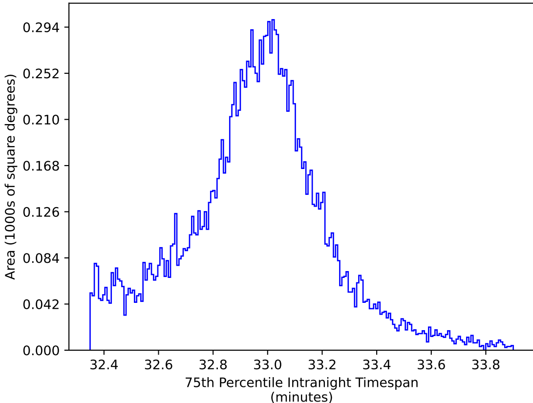
early_ss_template_fpextra2.0_v3.4_10yrs WFD y band: 75th Percentile Intranight Timespan
