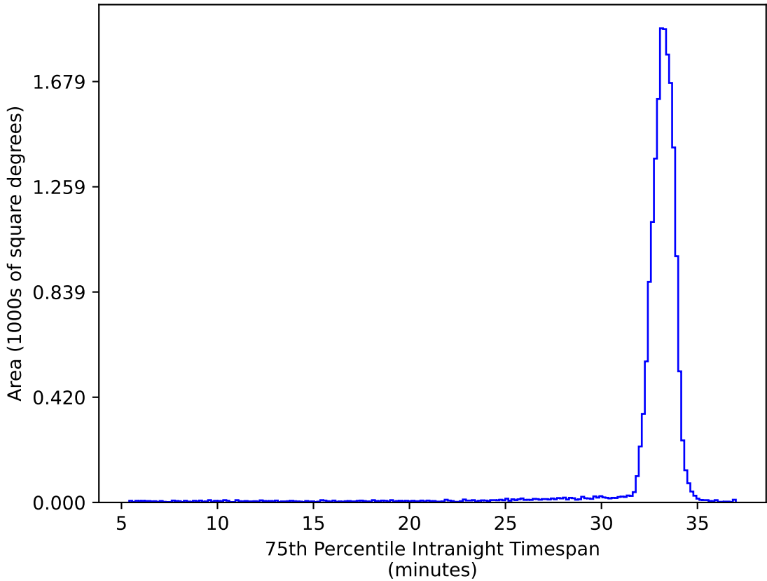
early_ss_template_fpextra2.0_v3.4_10yrs WFD ug bands: 75th Percentile Intranight Timespan
