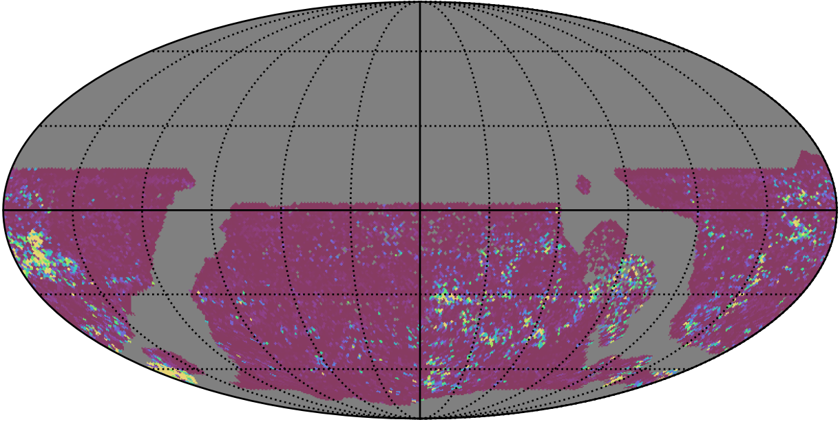
early_ss_template_fpextra2.0_v3.4_10yrs WFD u band: 75th Percentile Intranight Timespan
