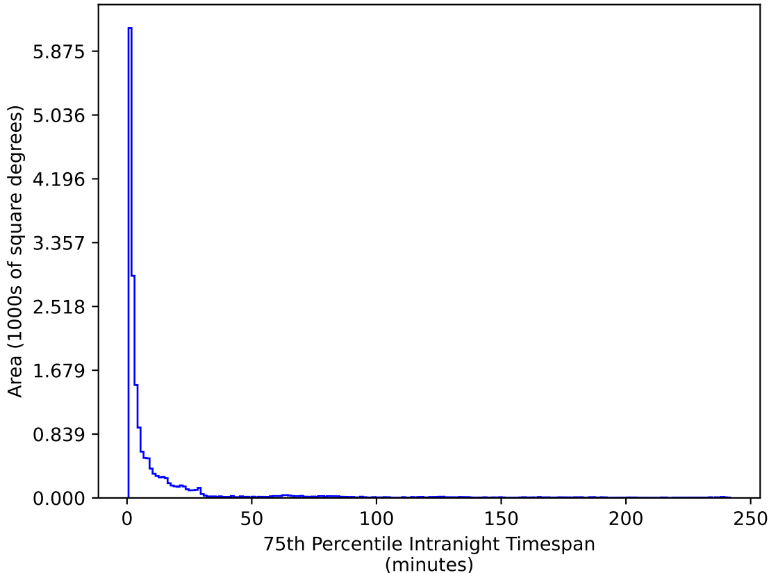
early_ss_template_fpextra2.0_v3.4_10yrs WFD u band: 75th Percentile Intranight Timespan
