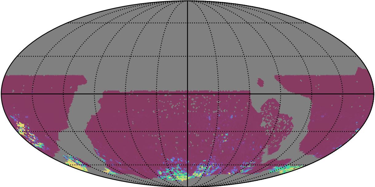
early_ss_template_fpextra2.0_v3.4_10yrs WFD ri bands: 75th Percentile Intranight Timespan
