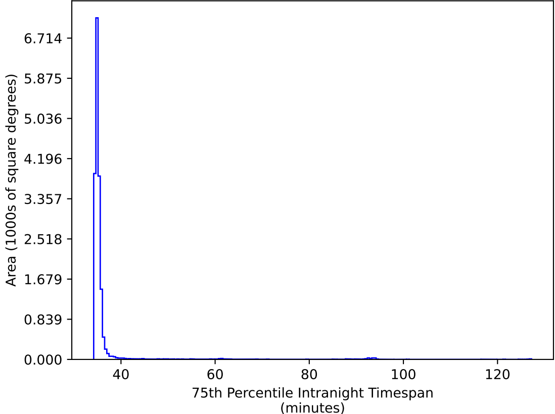
early_ss_template_fpextra2.0_v3.4_10yrs WFD ri bands: 75th Percentile Intranight Timespan
