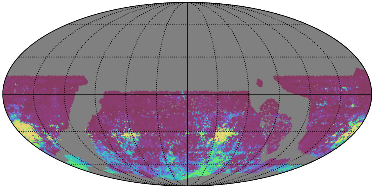
early_ss_template_fpextra2.0_v3.4_10yrs WFD r band: 75th Percentile Intranight Timespan
