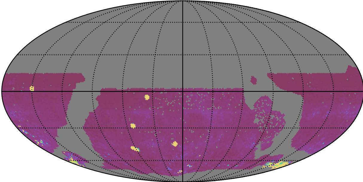
early_ss_template_fpextra2.0_v3.4_10yrs WFD iz bands: 75th Percentile Intranight Timespan
