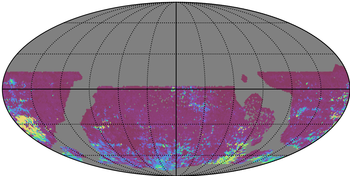
early_ss_template_fpextra2.0_v3.4_10yrs WFD i band: 75th Percentile Intranight Timespan
