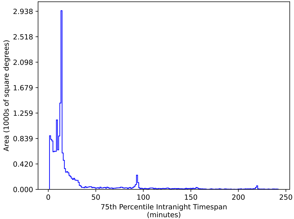
early_ss_template_fpextra2.0_v3.4_10yrs WFD i band: 75th Percentile Intranight Timespan
