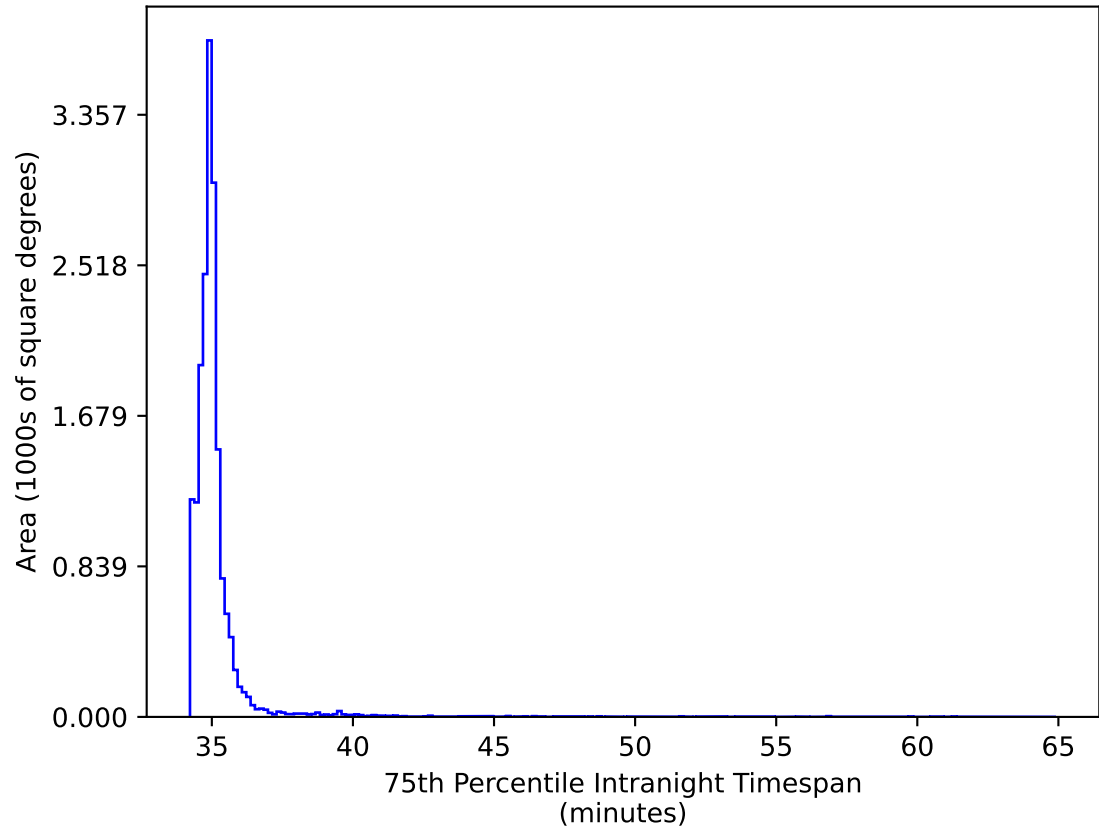
early_ss_template_fpextra2.0_v3.4_10yrs WFD gr bands: 75th Percentile Intranight Timespan
