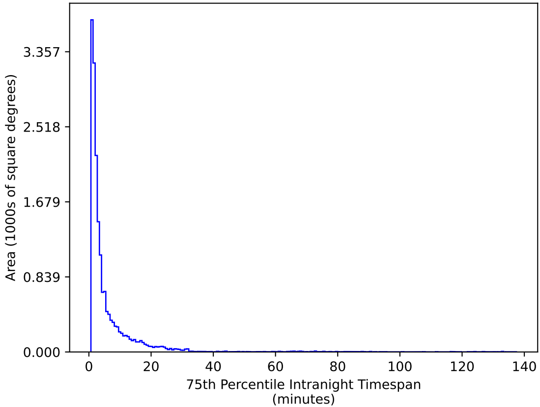
early_ss_template_fpextra2.0_v3.4_10yrs WFD g band: 75th Percentile Intranight Timespan
