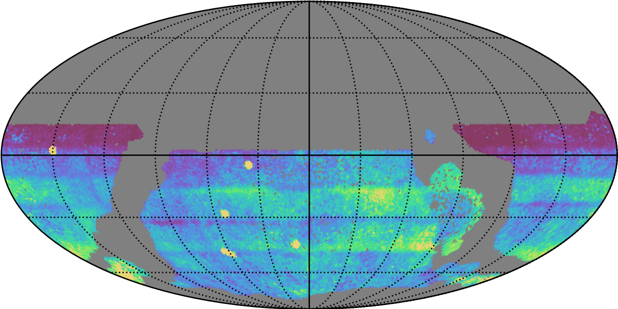
early_ss_template_fpextra2.0_v3.4_10yrs WFD all bands: 75th Percentile Intranight Timespan
