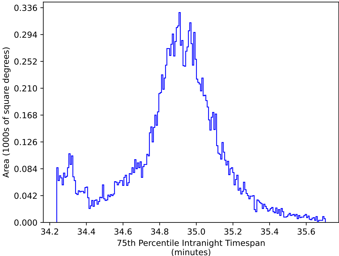
early_ss_template_fpextra2.0_v3.4_10yrs WFD all bands: 75th Percentile Intranight Timespan
