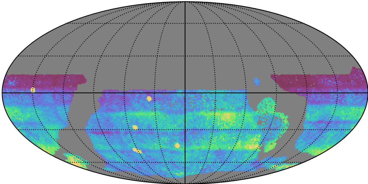
early_ss_template_fpextra2.0_v3.4_10yrs WFD: 75th Percentile Intranight Timespan
