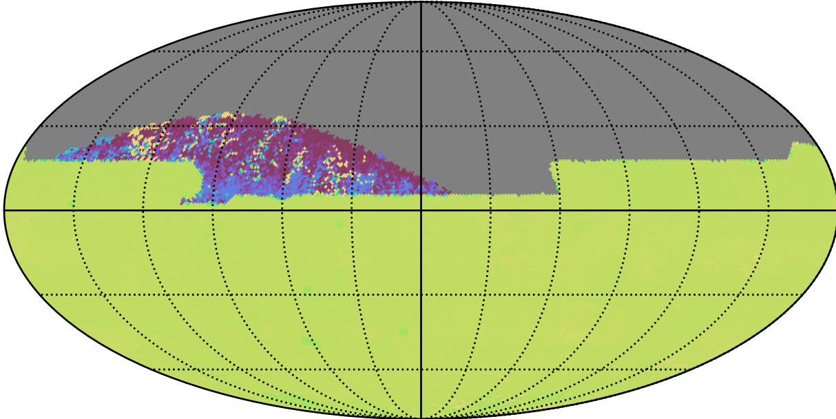
early_ss_template_fpextra2.0_v3.4_10yrs All sky zy bands: 75th Percentile Intranight Timespan
