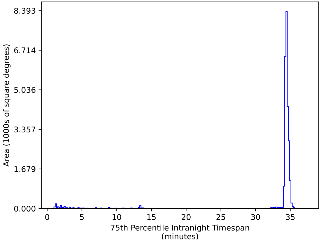
early_ss_template_fpextra2.0_v3.4_10yrs All sky zy bands: 75th Percentile Intranight Timespan
