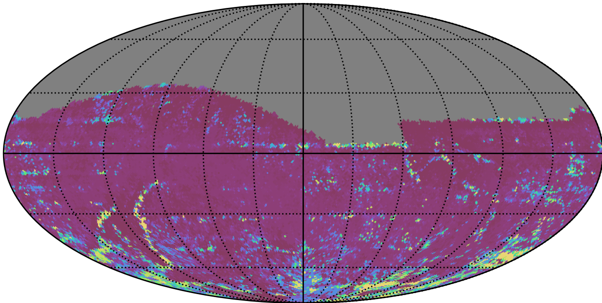
early_ss_template_fpextra2.0_v3.4_10yrs All sky z band: 75th Percentile Intranight Timespan
