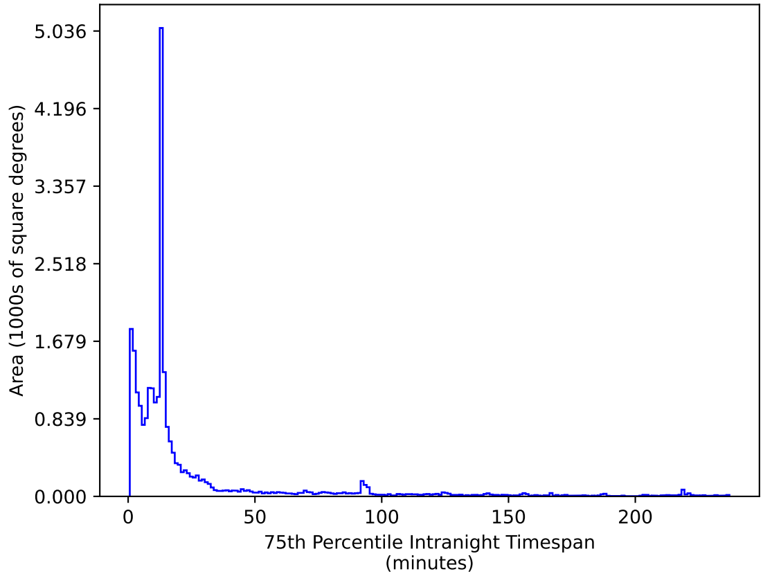
early_ss_template_fpextra2.0_v3.4_10yrs All sky z band: 75th Percentile Intranight Timespan
