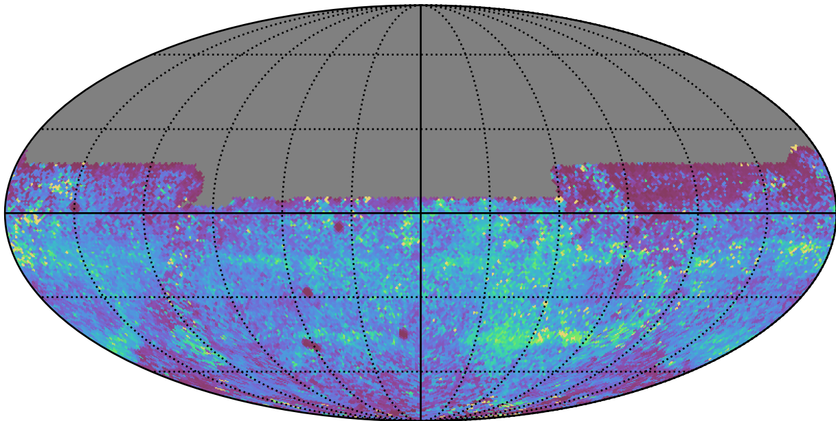
early_ss_template_fpextra2.0_v3.4_10yrs All sky y band: 75th Percentile Intranight Timespan
