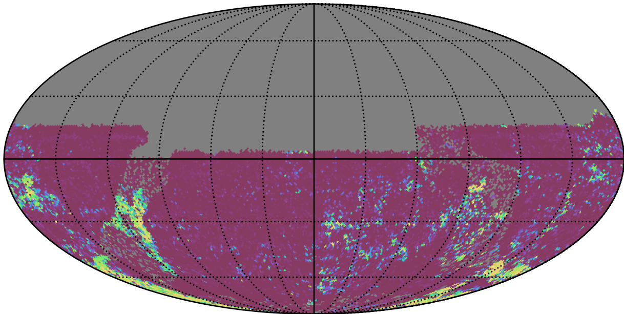
early_ss_template_fpextra2.0_v3.4_10yrs All sky u band: 75th Percentile Intranight Timespan
