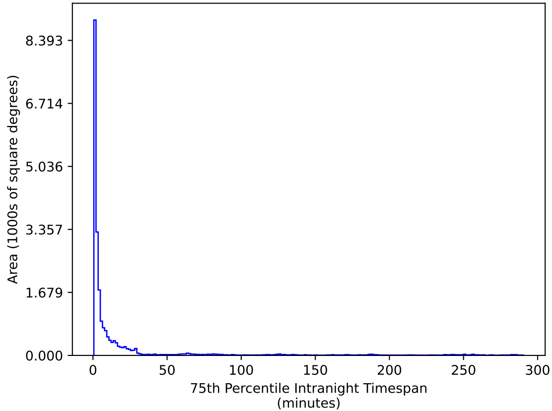
early_ss_template_fpextra2.0_v3.4_10yrs All sky u band: 75th Percentile Intranight Timespan
